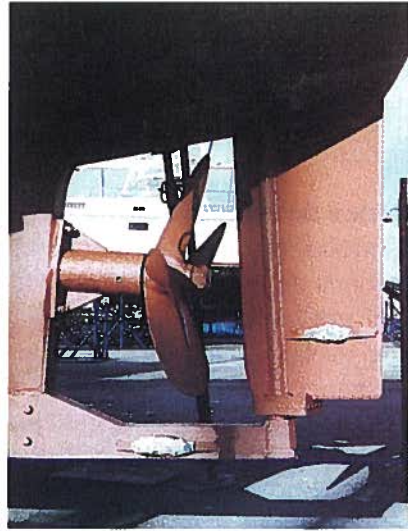
Timón semicompensado
