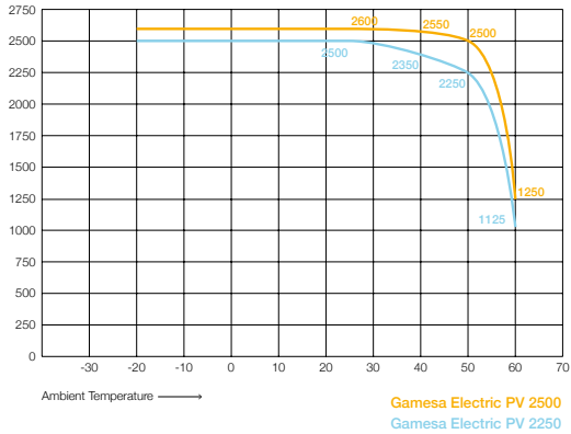
Efficiency PV 2500
