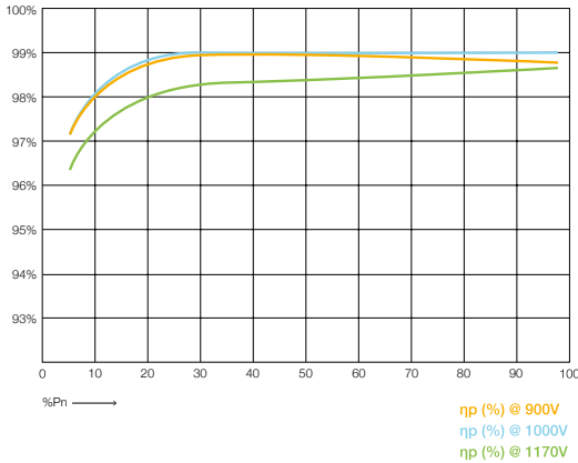
Efficiency PV 2250
